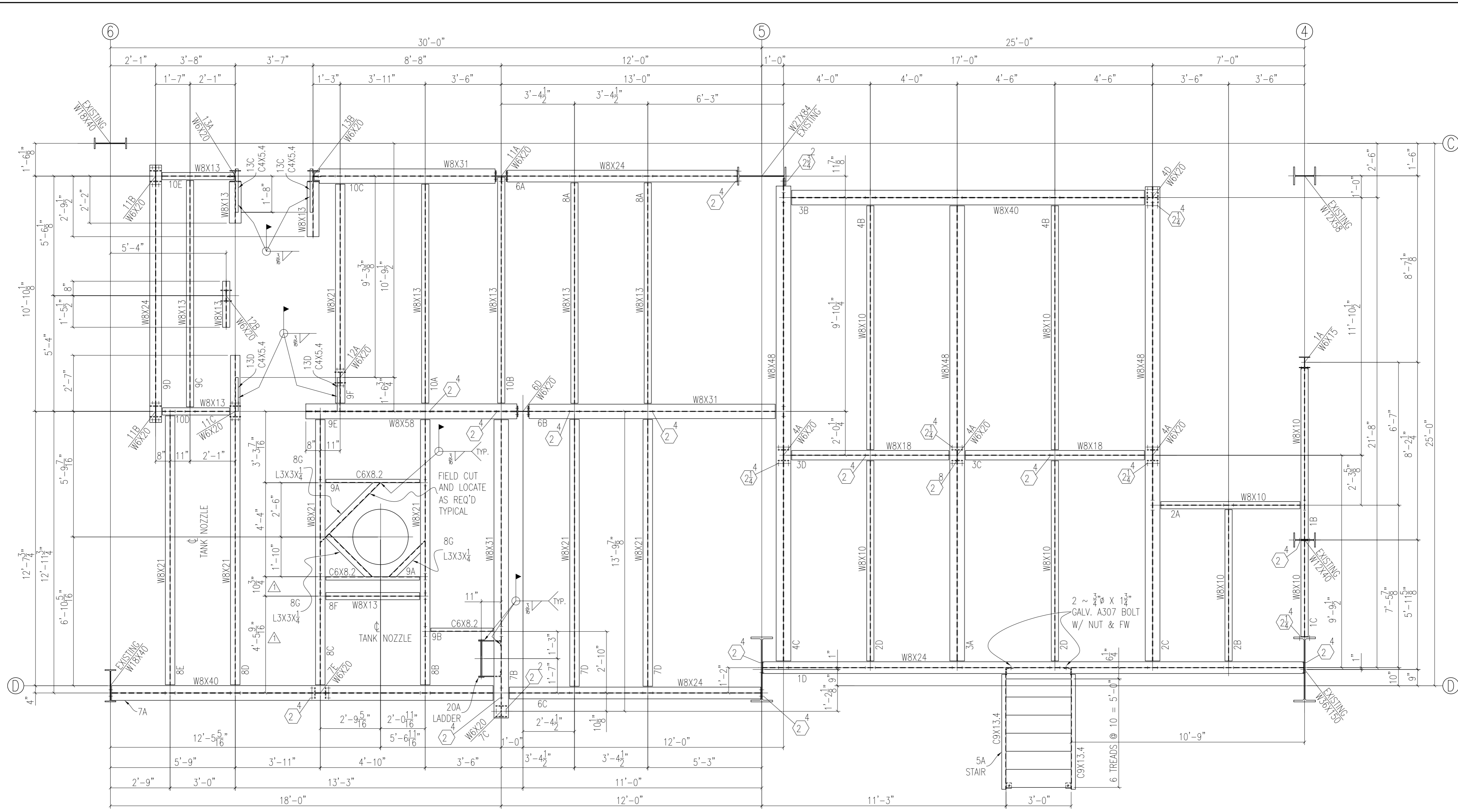
PLATFORM PLAN TOS EL= 105'-0" U/N TOS EL = 105'-4" @ THE C4X5.4 U/S OF BASE PLATE EL = 100'-5 1/2" TYPICAL U/N U/S OF BASE PLATE AT COLUMNS 12A & 12B EL = 97'-9 1/2"
